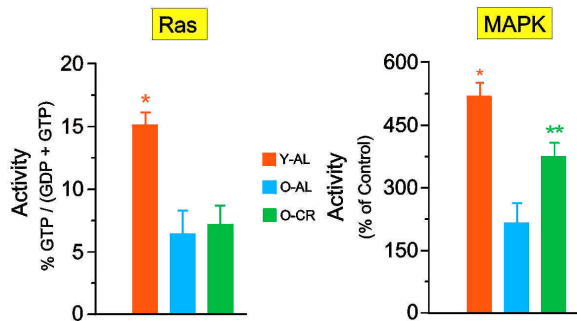
Figure 1. Effect of caloric restriction and aging on the induction of Ras and MAPK activation in T cells from rats. Splenic T cells from control (AL) young and old rats or caloric restricted (CR) old rats were incubated with or without Con A for 10 min to measure Ras activity or for 15 min to measure MAPK activity. The Ras activity is expressed as the percentage ratio of GTP-p21 ras over total (GDP-p21 ras plus GTP-p21 ras ). The data for MAPK activity is expressed as the percentage of activity in Con A (CA)-stimulated cells relative to the unstimulated cells. Each point represents the mean \pm SD for data obtained from three experiments (for the Ras activity) or from four experiments (for the MAPK activity) and each experiment was pooled from two rats. Data were taken from Pahlavani, M.A and D.A. Vargas (35). * The value for young rats was significantly different from the values for the control old rats at the p < 0.001 . ** The value for caloric restricted old rats was significantly different from the value for the age-matched control at the p < 0.05 .
