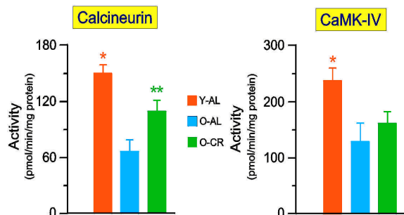
Figure 2. Effect of caloric restriction and aging on the induction of calcineurin (CaN) and CaMK-IV activities in T cells from rats. Splenic T cells from control (AL) young and old rats or caloric restricted (CR) old rats were cultured in the presence or absence of Con A. After 5 to 10 minutes of incubation, cells were lysed and the protein extracts were assayed for CaN phosphatase activity and CaMK-IV activity. Each point represents the mean \pm SD for data obtained from four experiments for the CaN assay, and three experiments for the CaMK-IV assay, each experiment was pooled from two rats. Data were taken from Pahlavani, M.A and D.A. Vargas (35). * The value for young rats was significantly different from the values for the control old rats and caloric restricted old rats at p < 0.05 . ** The value for caloric restricted old rats was significantly different from the value for the age-matched control at p < 0.05 .
