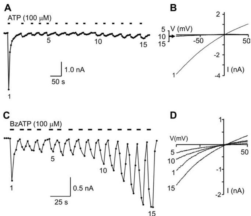
Figure 4. Repeated application of nucleotides to rabbit osteoclasts induces an initial P2X 4 current that desensitizes, followed by an activity-dependent P2X 7 current. Representative traces from osteoclasts stimulated either with 100 μM ATP (upper row) or 100 μM BzATP (lower row). Whole-cell currents (left) were recorded at a holding potential of -30 mV (pipette solution contained Cs + to block K + currents). Bars above the current traces represent agonist applications. Voltage ramps were applied to obtain current-voltage curves (right) at the times indicated by the numbers. Nucleotide-induced currents were obtained by subtraction of the basal, resting current. (A) Initial stimulation of an osteoclast with 100 μM ATP elicited a large inward P2X 4 current, whereas successive applications of ATP resulted in little response, due to P2X 4 desensitization. (B) The corresponding current-voltage curves for this cell indicate that the initial ATP-induced current had a reversal potential near 0 mV, as expected for the non-selective cation pore of P2X 4 . (C) Another osteoclast was stimulated with the more potent P2X 7 receptor agonist BzATP (100 μM). After the initial response, successive stimulations led to the progressive development of an inward current of increasing amplitude. The results are consistent with initial activation of P2X 4 receptors, followed by their desensitization and progressive recruitment (priming) of P2X 7 receptors with successive stimulations. (D) The current-voltage curves for the cell in panel C indicate that both the initial current that desensitizes (the P2X 4 current) and the progressively developing current (the P2X 7 current), had reversal potentials near 0 mV. Reproduced with permission from (34).
