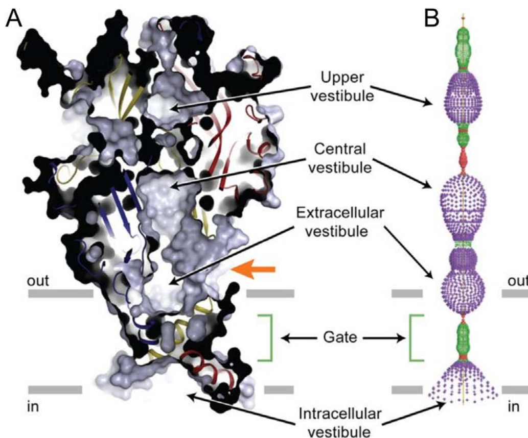
Figure 1. Crystal structure of Danio rerio P2X 4 receptor. (A) Sagittal section, showing a closed conformation of the pore. The gate is located about halfway across the membrane bilayer. Four vestibules (upper, central, extracellular and intracellular) are located on the molecular three-fold axis, with the extracellular vestibule connected to the bulk solution through a fenestration (orange arrow). (B) Pore-lining surface. Each color represents a different radius range measured from the receptor centre (red: <1.15 Å, green: 1.15–2.3 Å, and purple: >2.3 Å). Reproduced with permission from (32).
