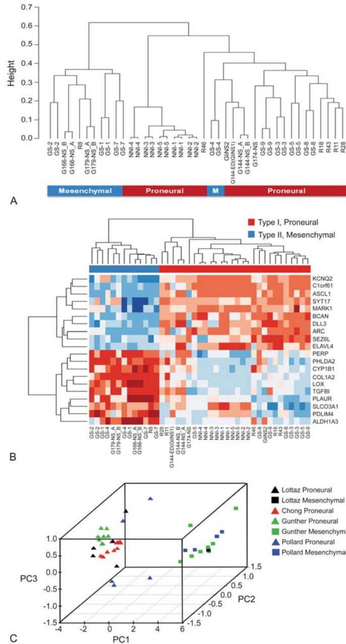
Figure 3. Vitrified GBM-initiating cells could be grouped into two subtypes and were differentially regulated by Proneural genes and TGFbeta signaling pathways. An integrated non-parametric analysis of gene expression in 4 glioma stem cell datasets is shown: (A) An unbiased whole transcriptome (all commonly expressed genes between Illumina & Affymetrix platforms) hierarchical clustering based on a non-parametric rank-sorted binning (500 quantile bins) of each expression dataset, using a spearman rank correlation distance metric and complete linkage. Grouping of samples into Type I (Proneural) represented as red bar and Type II (Mesenchymal) represented as blue bar, based on classification by Lottaz et al. (17). (B) Heatmap clustering of 4 BTSC datasets based on a signature of 20/24 genes (4 genes: NGC, GLUR2, SOX11 and unknown 213484_at were not adequately represented on the Illumina Human ref8v2 gene array) published by Lottaz et al. (17). Clustering was based on a spearman rank correlation distance of a non-parametric rank sorted binning (500 bins/sample) of gene level averaged expression data for each dataset. (C) 3D principal component analysis (PCA) of spearman rank correlation distance between the models in each of the BTSC datasets. The first 3 principal components are shown capturing more than 90 percent of the total variance in the dataset. Plotting symbols demarcate Type I (Proneural, ▲) and Type II (Mesenchymal, ■) BTSC subtypes, while colors demarcate the different sources of BTSCs: Red, Chong et al. , (15); Green, Gunther et al. , (53); Black, Lottaz et al. , (17) and Blue, Pollard et al. (16).
