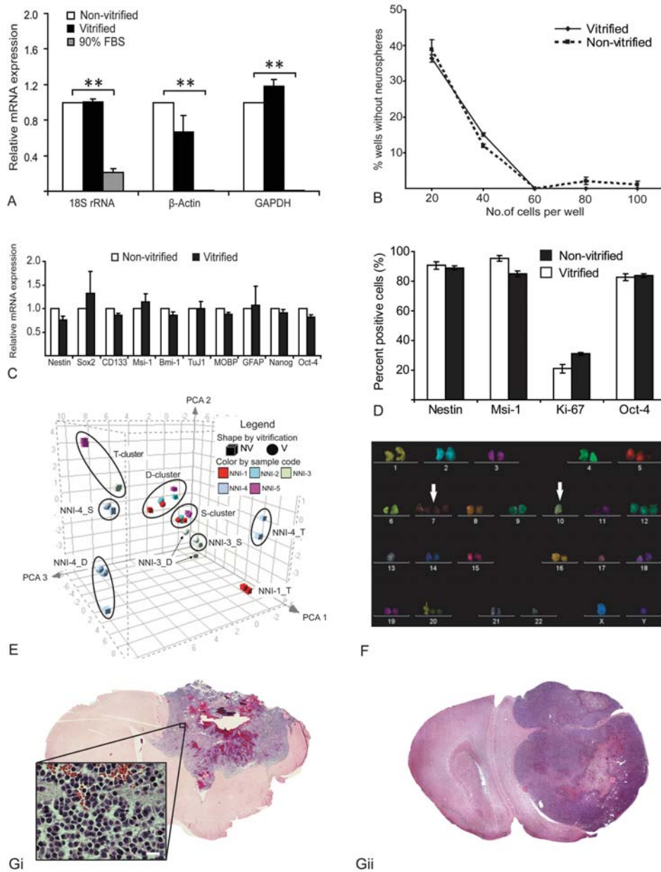
Figure 1. Vitri-fied GBM-initiating cells using low serum content preserved their BTSC frequency, gene expression, surface marker expression, karyotypic profile and created xenografts that recapitulated the original disease pathophysiology. (A) Cryopreservation with high serum content led to altered levels of several constitutively expressed genes upon thawing and re-culturing. Data were normalized against the hypoxanthine-guanine phosphoribosyltransferase (HPRT) gene. ** denotes p less than 0.01. (B) Vitri-fied cells preserved their BTSC frequency. (C) Vitri-fied BTSCs preserved mRNA levels of key stemness and differentiation genes. (D) Vitri-fied BTSCs preserved cell numbers expressing common stemness markers. (E) Principal component analysis map of BTSCs showed that vitri-fied and non-vitri-fied cells in each of stemness and differentiated states clustered together. BTSCs were genetically distinct from the primary tumor. Two BTSC lines (NNI-1_S in S cluster and NNI-4_S) exhibited distinct transcriptomic profiles even though they showed identical GBM histology of their primary tumors. BTSC lines from a previous manuscript (15) are re-named here for simplicity: NNI-1 replaces S0305, NNI-2 replaces S0405, NNI-3 replaces S0805, NNI-4 replaces S0306, NNI-5 replaces S0807. (F) BTSCs preserved karyotypic hallmarks of GBM, notably amplification of chromosome 7 and loss of chromosome 10. (Gi) Anaplastic oligoastrocytoma BTSC intracranial xenograft exhibited extensive infiltration, hemorrhaging and displayed the typical “fried egg” morphology and “chicken wire” patterning of stroma. Scale bar represents 20 microns. (Gii) Intracranial xenograft established from serum-grown U87MG displayed spatially constrained, well-lined tumor margins. Figures C, D and F were reproduced with permission from, (15). Figures B and E were adapted from data obtained in (15).
